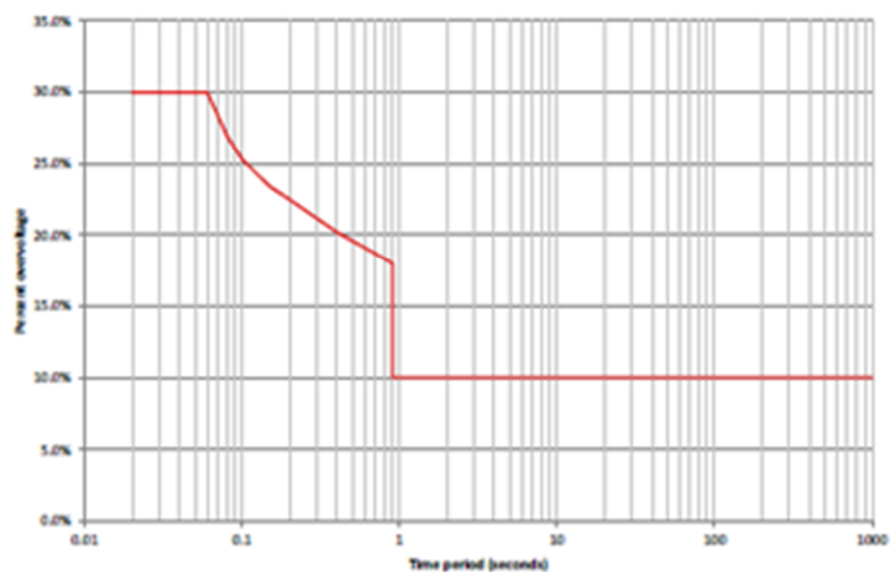
Figure 4 – Over voltage limit for contingency events
