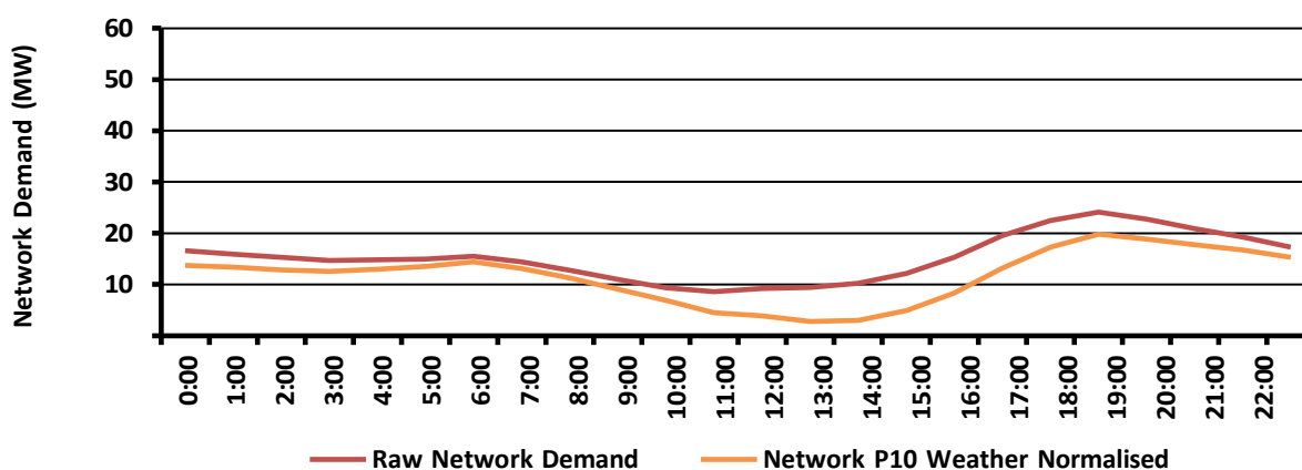
Figure C6 – Alice Springs Min Day Load Profile
