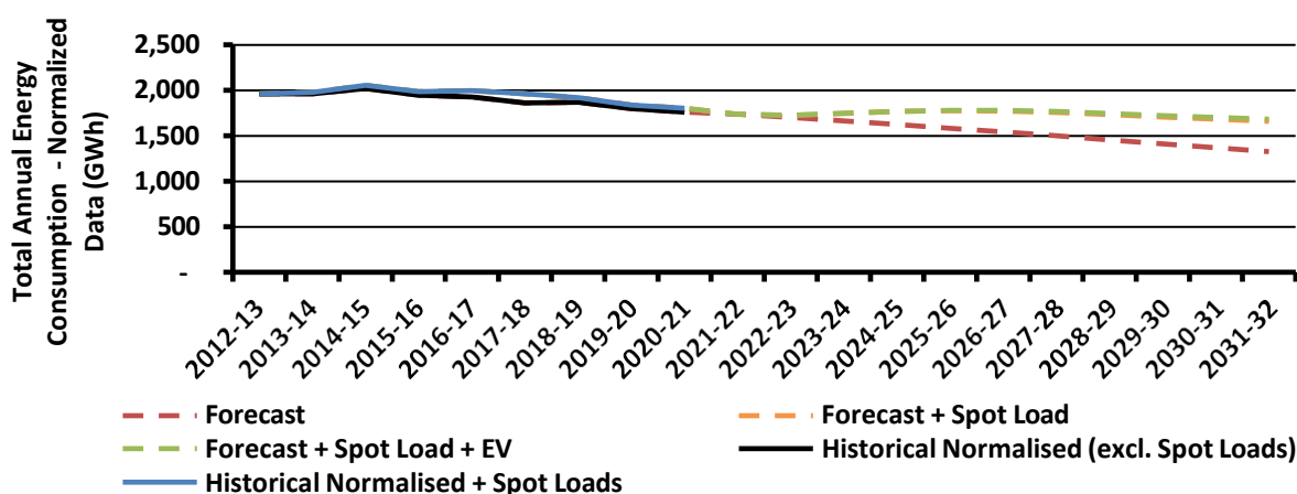
Figure 15 – NT Total, Historical and Forecast P50 Energy Consumption, Spot Loads and EVs
