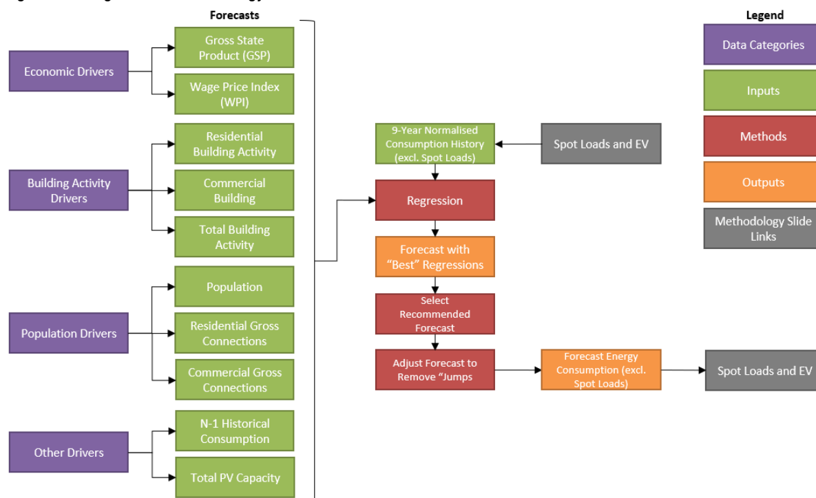
Figure 2 – Regression Methodology Overview
