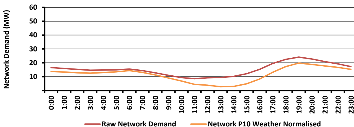
Figure C6 – Alice Springs Min Day Load Profile
