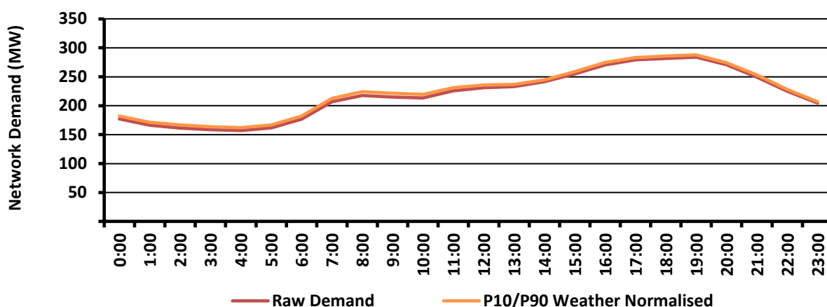
Figure C2 – DKIS Peak Day Load Profile
