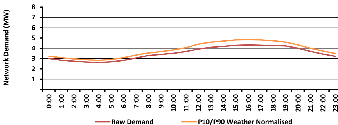
Figure C7 – Tennant Creek Average Day Load Profile
