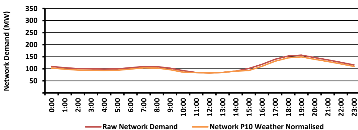
Figure C3 – DKIS Min Day Load Profile
