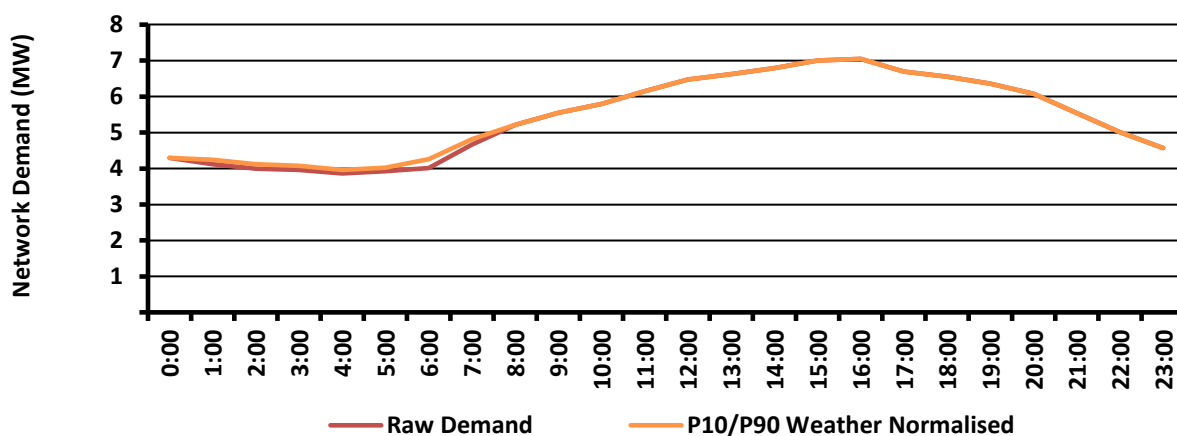
Figure C8 – Tennant Creek Peak Day Load Profile
