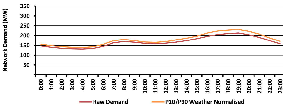
Figure C1 – DKIS Average Day Load Profile
