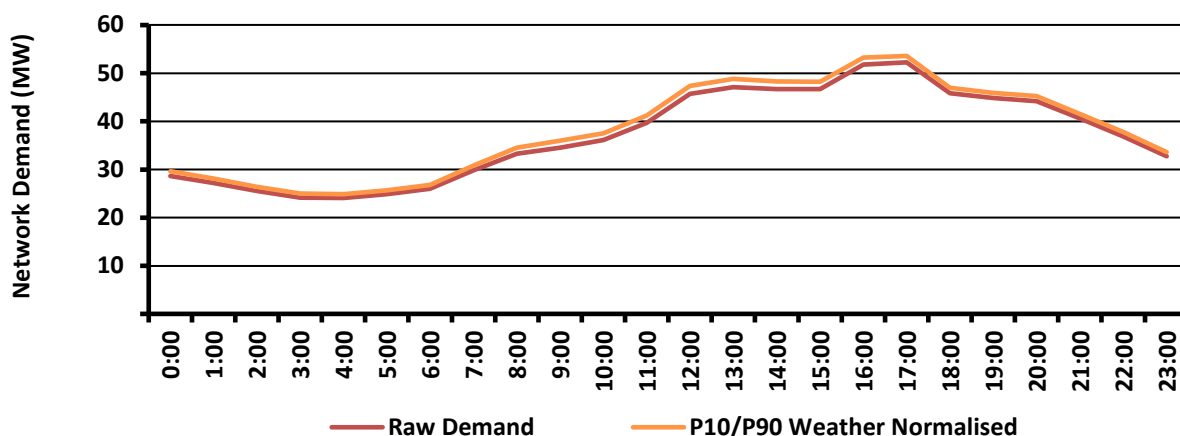
Figure C5 – Alice Springs Peak Day Load Profile
