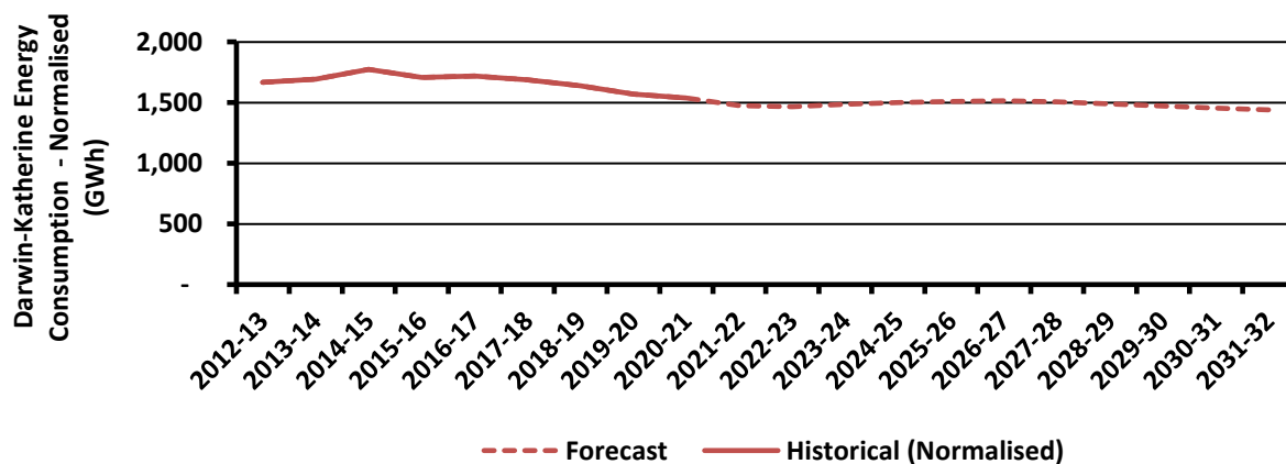
Figure 16 – DKIS, Historical and Forecast P50 Energy Consumption
