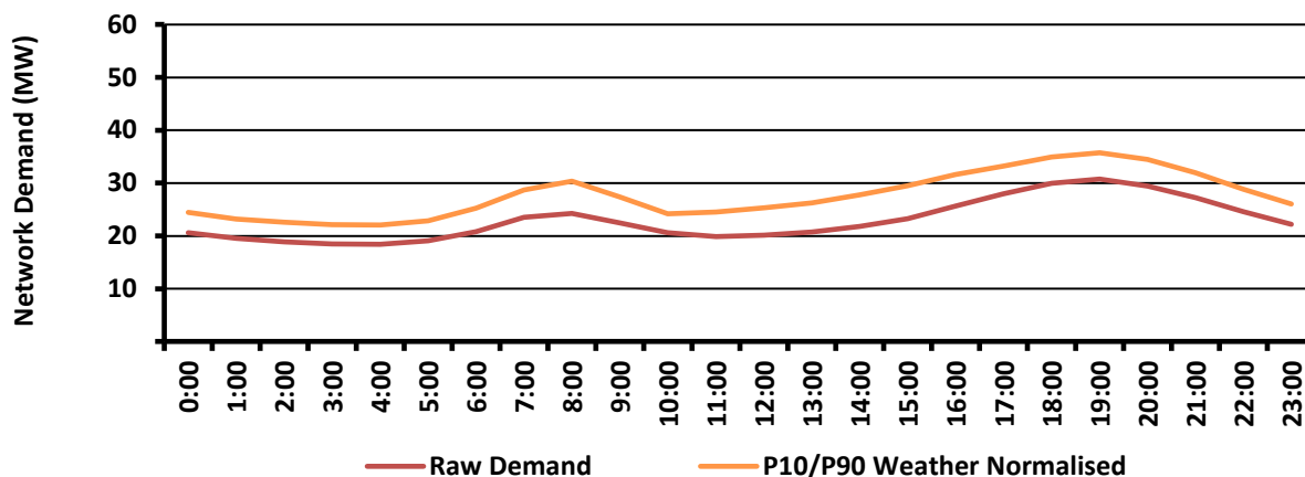
Figure C4 – Alice Springs Average Day Load Profile
